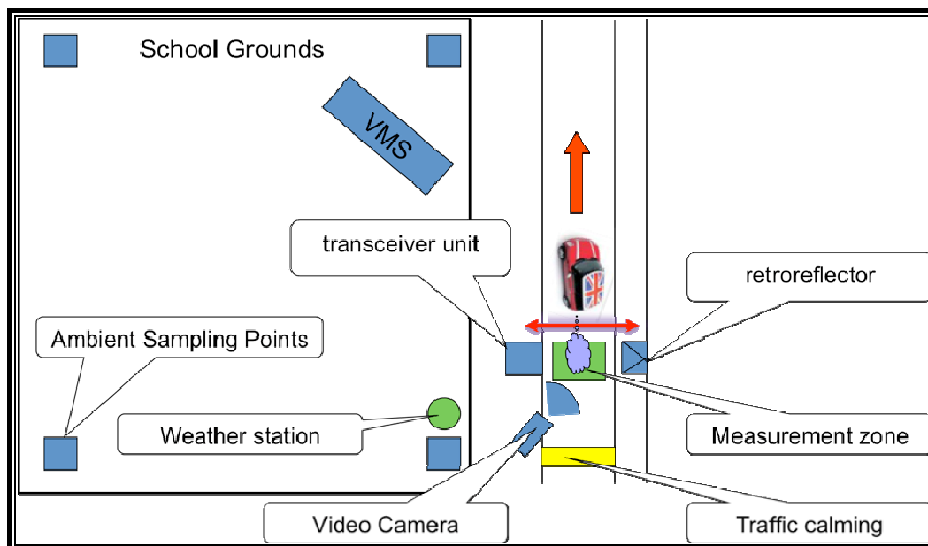
Figure 9 CIVITAS education project proposed pollution monitoring equipment layout
